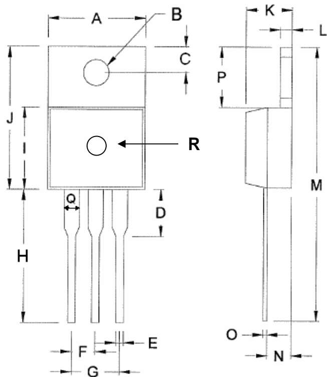
TO-220
